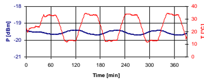
temperature drift of output level
